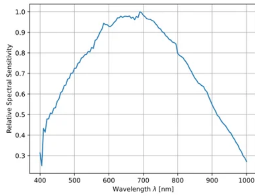
IMX900 Sensor QE Curve
