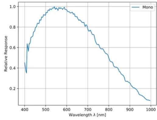
IMX546 Sensor QE Curve
