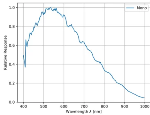
GMAX2505 Sensor QE Curve
