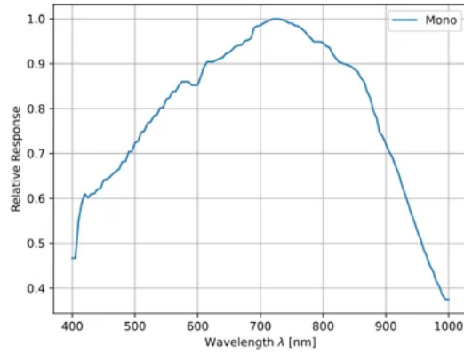
IMX676 Sensor QE Curve
