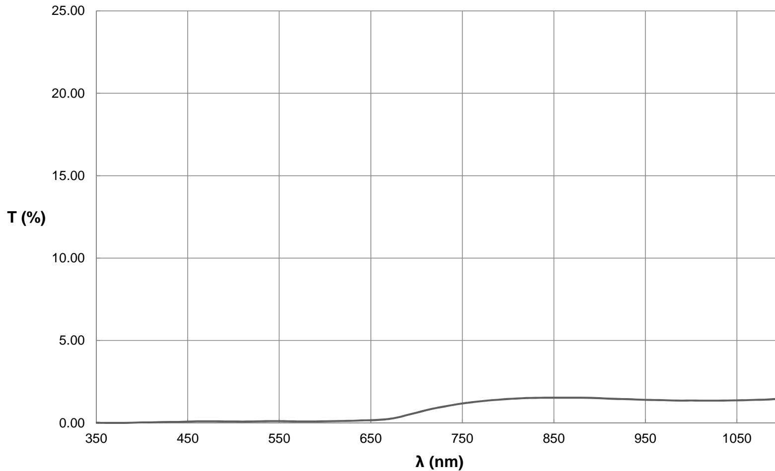
Machine Vision ND 3.0 Filter, 0.1% Average Transmission (425nm-675nm) FOR REFERENCE ONLY
