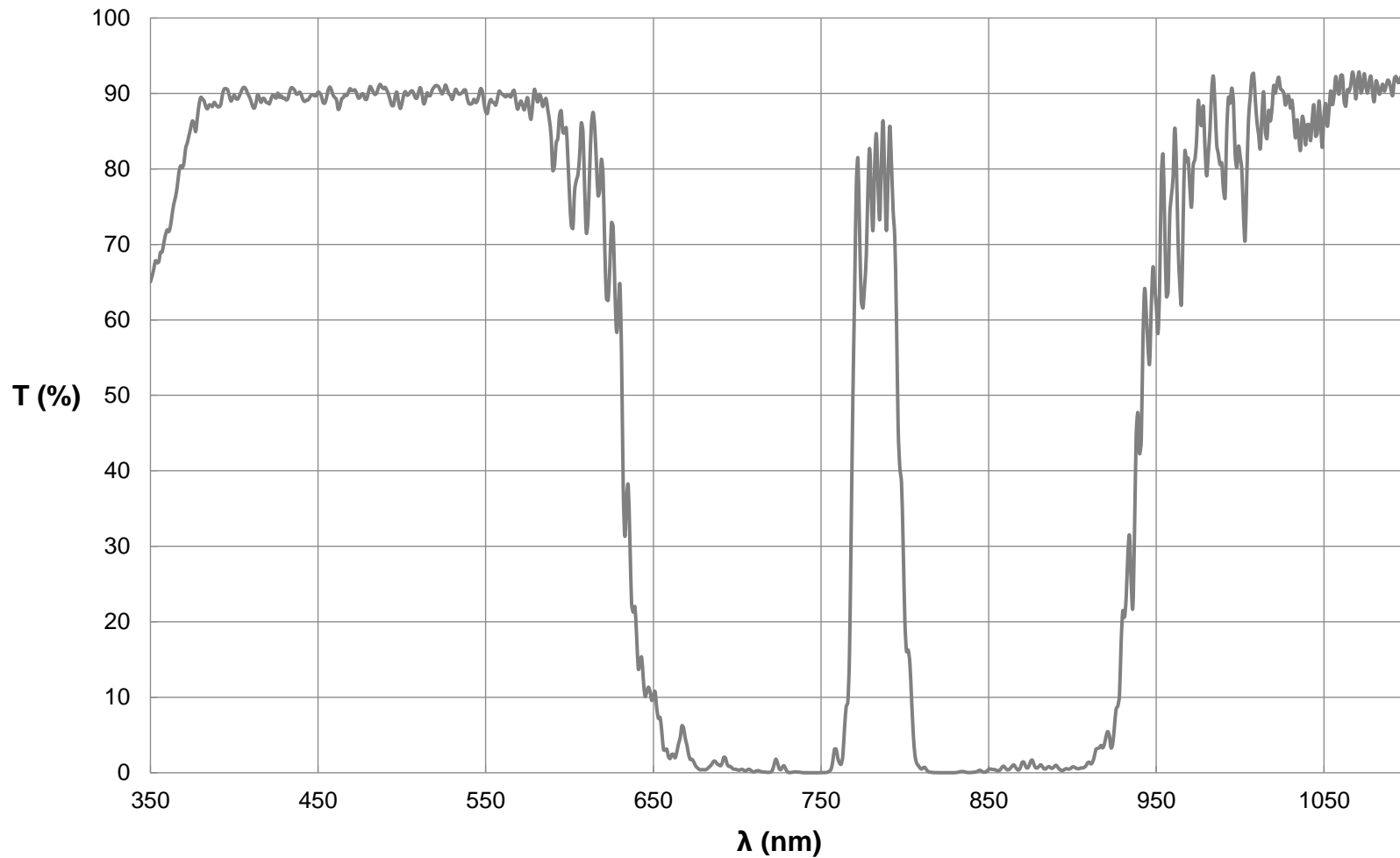
Everix Ultra-Thin Bandpass Filter, 785nm, OD 2.0 FOR REFERENCE ONLY
