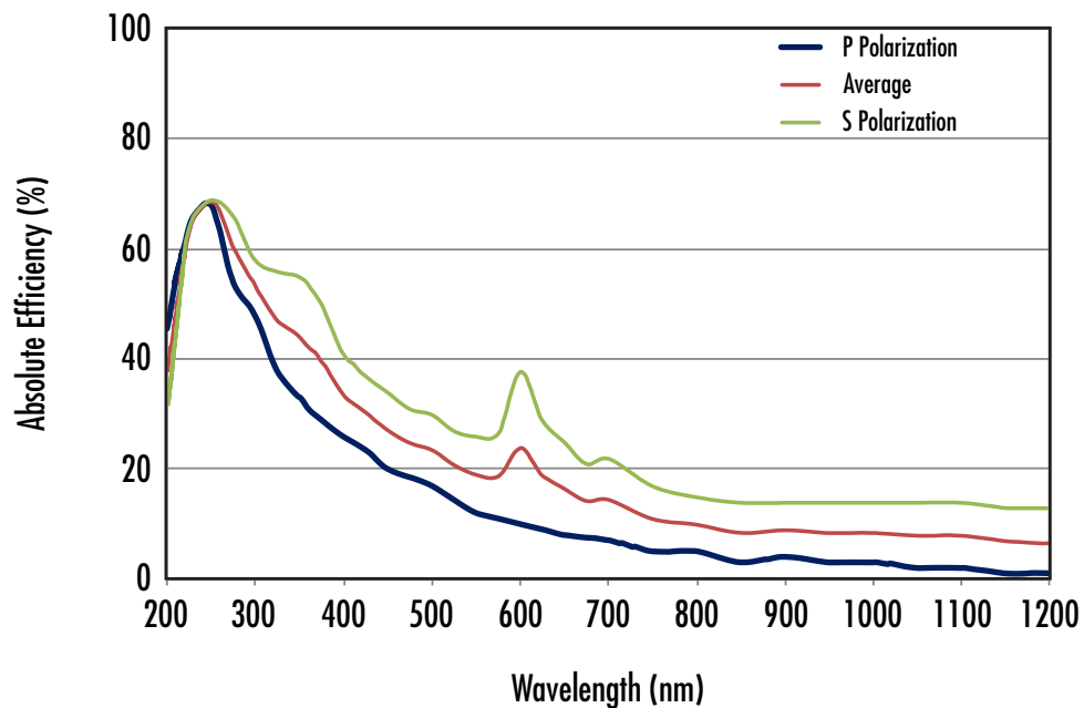
1200 Grooves/mm, UV Holographic Grating Absolute Efficiency
