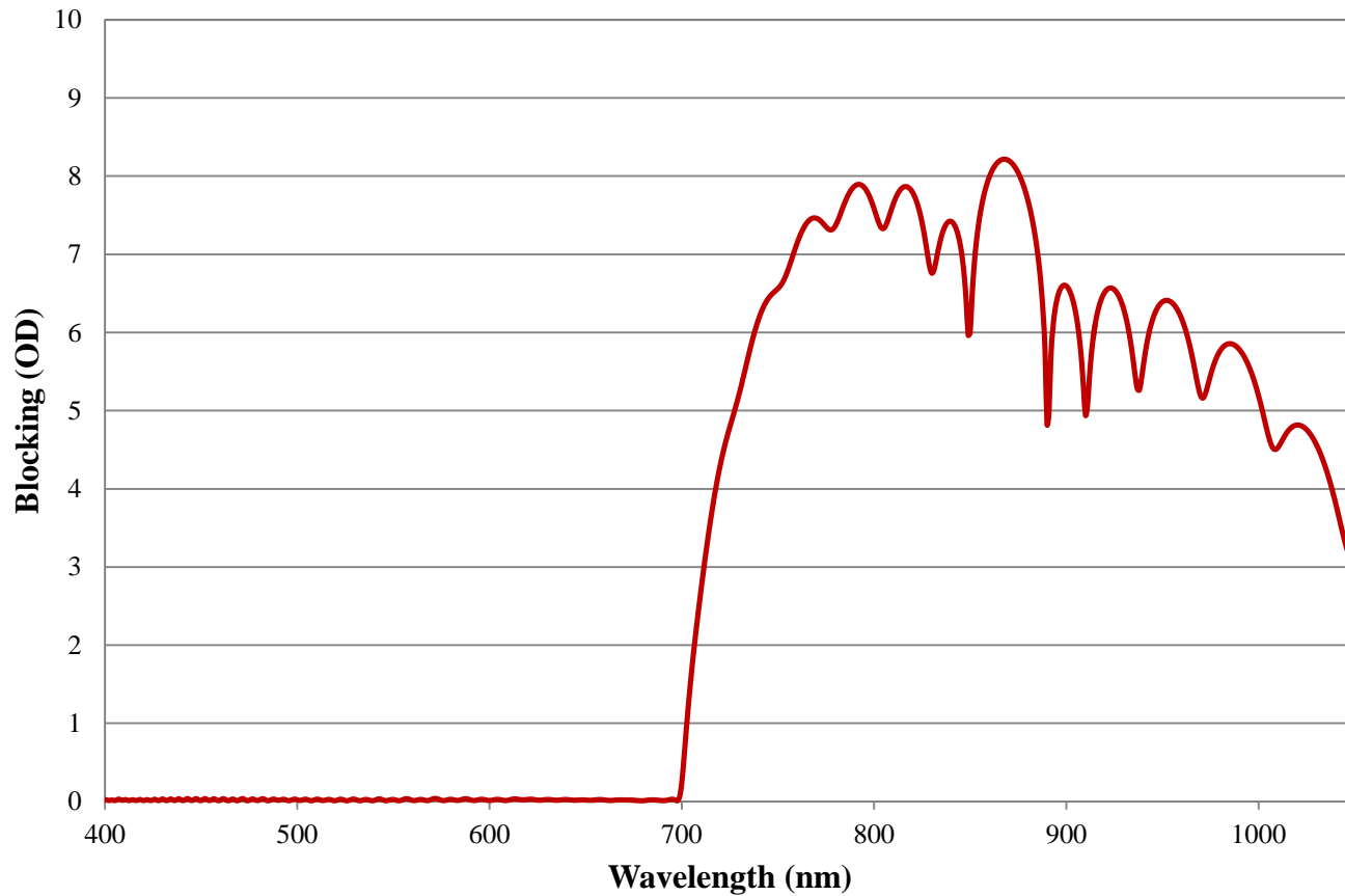
700nm Techspec® Shortpass Filter: OD >4.0 Coating Performance FOR REFERENCE ONLY
