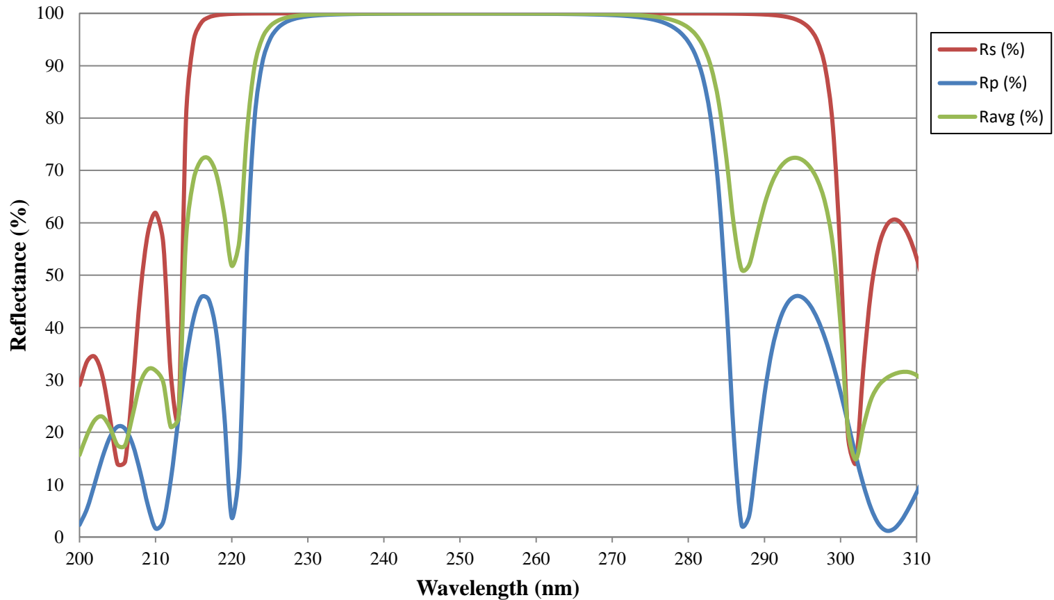
248nm 45° AOI - Excimer Laser Line Mirror Coating Performance FOR REFERENCE ONLY
